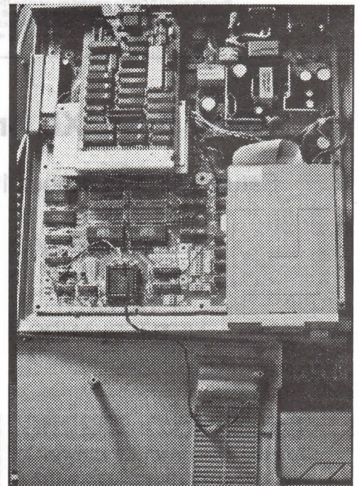
Above: The QVME Card: High quality construction. Below: The QVME Card fits nicely into the Atari STe.
